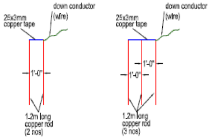
2 ROD ARRANGEMENT
