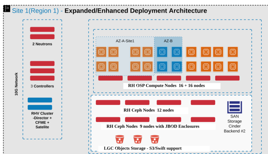
Figure 1: Current LGC 2 Site1 Architecture
